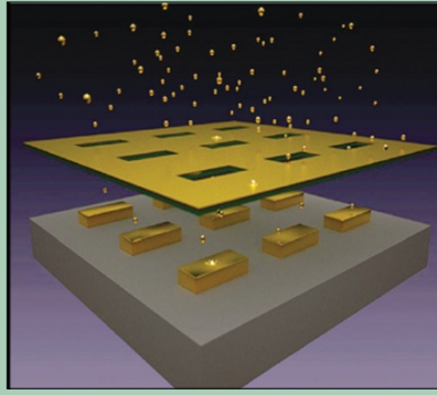
Nanostencil lithography: ERC researchers have developed a new way to make large numbers of plasmonic nanorod antenna arrays using nanostencil lithography. The arrays have the same optical properties as those engineered by conventional electron lithography and could revolutionize light sensing.
